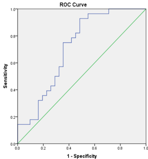
Figure 4. ROC curve of tissue miR-361 levels for molecular differentiation of tumor from non-tumor samples. The area under the ROC curve for this analysis was 0.71 (95% CI: 0.58-0.84)
