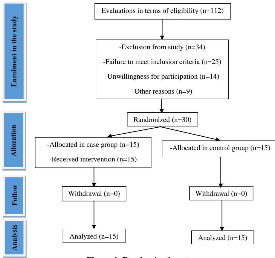
Figure 1. Randomization steps
