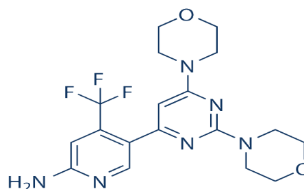
Fig. 1. Chemical structure of Buparlisib.
