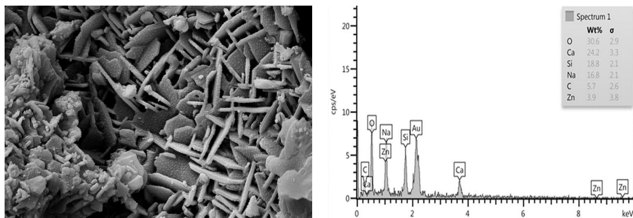
Figure 3. SEM-EDS analyses
