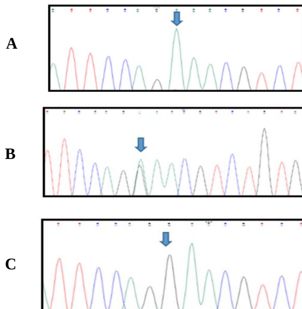
Figure 3. Sequencing results for AA (A), AG (B), and GG (C) genotypes
