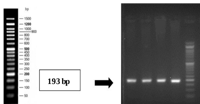
Figure 1. Electrophoresis on 2% agarose gel for a selection of PCR products from patients and a 50-bp DNA ladder. (The molecular size marker is shown in the figure)
