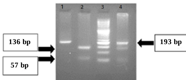
Figure 2. Electrophoresis on 2% agarose gel for the enzyme-digested products. Lane 1: AA genotype, Lane 2: GG genotype, Lane 3: 50-bp DNA ladder, Lane 4: AG genotype
